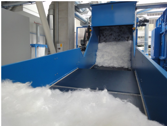
Photo 3: Rough fibre opening
